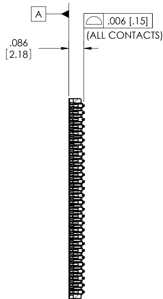
SECTION E-E
